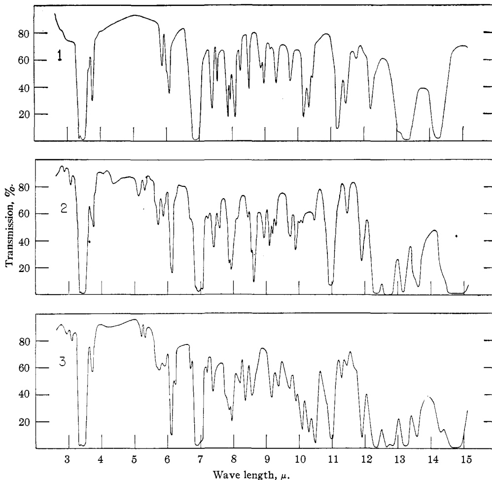
Fig. 2.—Infrared absorption spectra: Curve 1, cycloöctene prepared by partial hydrogenation of cycloöctatetraene; curve 2, 1,3-cycloöctadiene (V), n^{25}_D 1.4908, prepared by dehydrohalogenation of I; curve 3, 1,3-cycloöctadiene (V), n^{25}_D 1.4940, prepared from IV.
